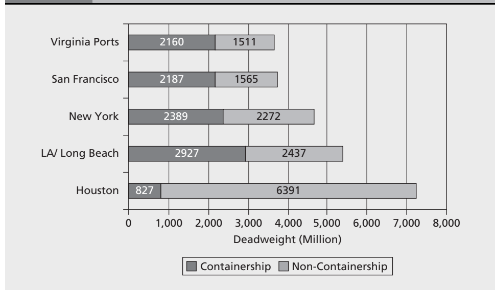
FIGURE 14-4A Top Vessel Calls by U.S. Port, 2011
